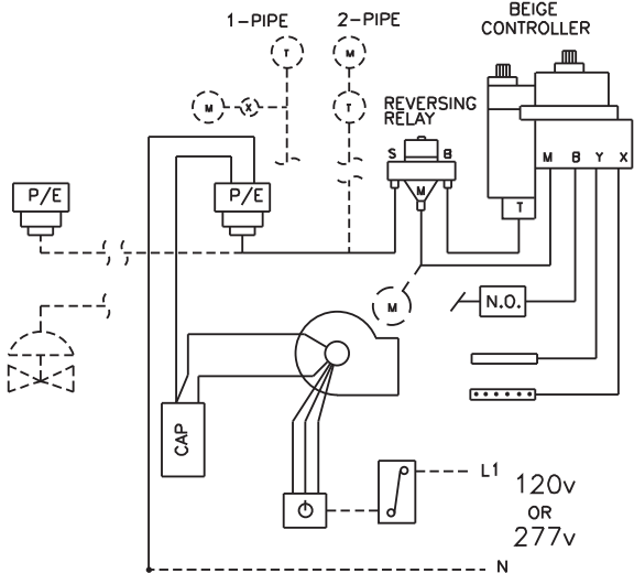
REVERSE-ACTING THERMOSTAT
