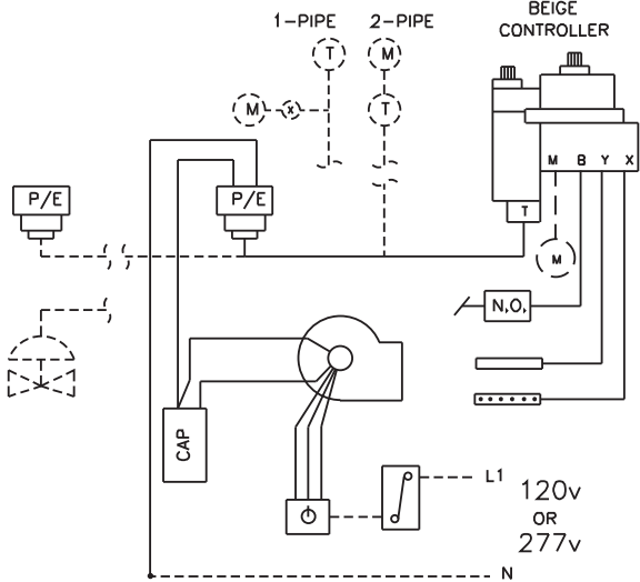
DIRECT-ACTING THERMOSTAT
