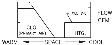
REVERSE-ACTING THERMOSTAT
