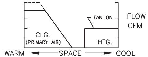
REVERSE-ACTING THERMOSTAT
