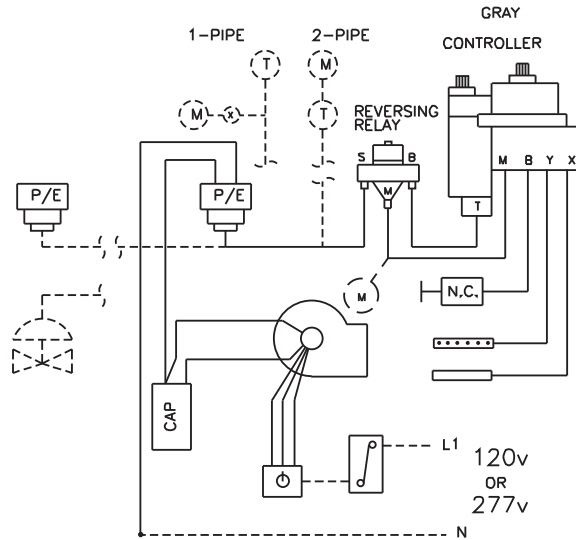
DIRECT-ACTING THERMOSTAT
